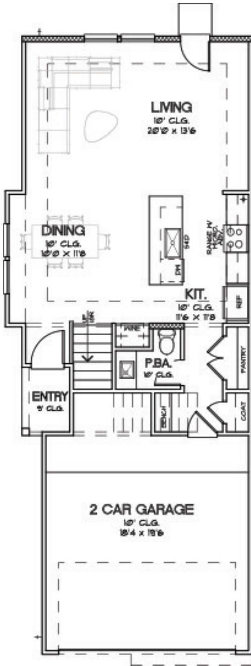
FIRST FLOOR
