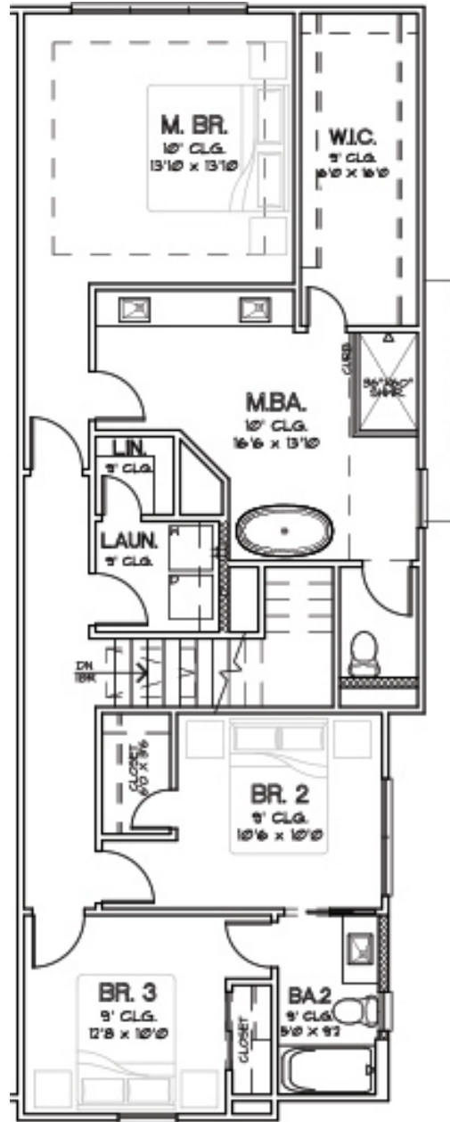
SECOND FLOOR
