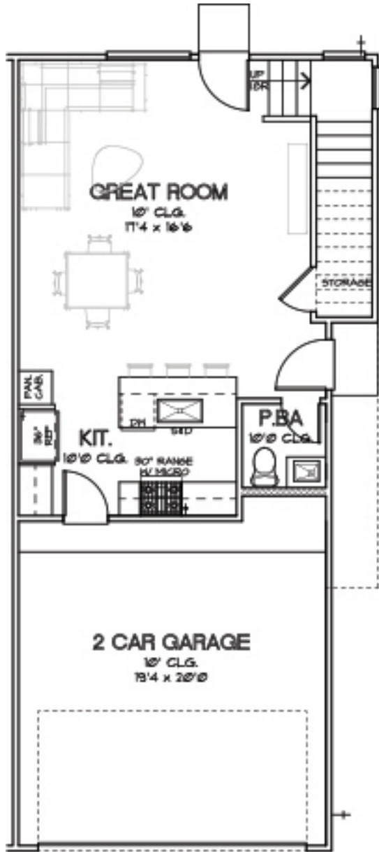
FIRST FLOOR
